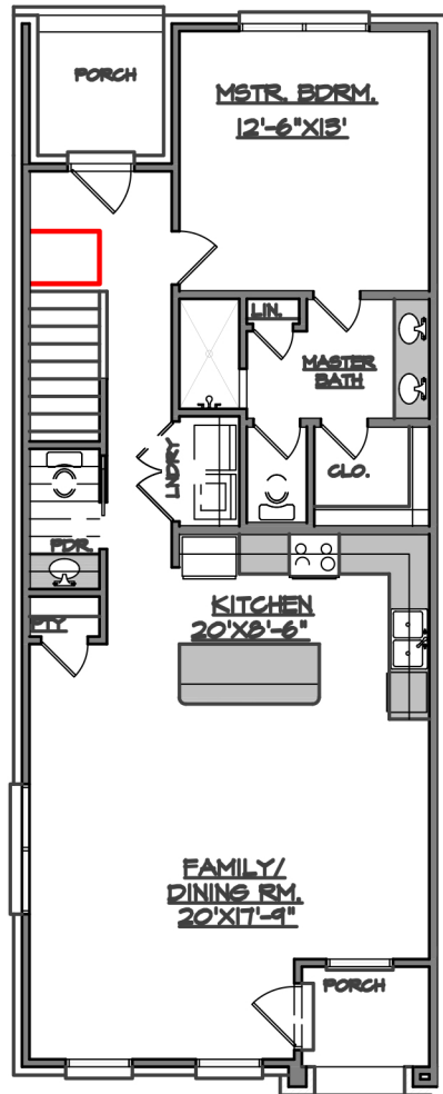
FIRST LEVEL FLOOR PLAN LEFT UNIT
