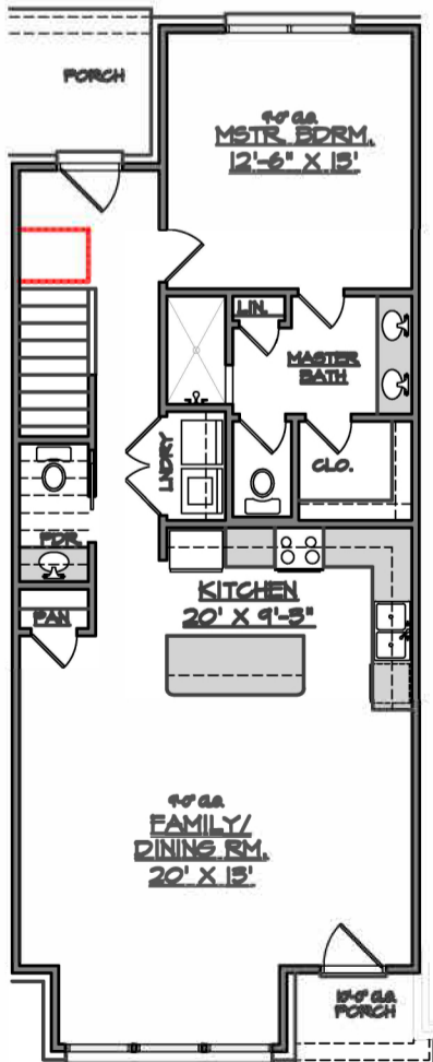
FIRST LEVEL FLOORPLAN BAY UNIT
