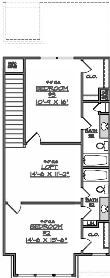
SECOND LEVEL FLOORPLAN BAY UNIT
