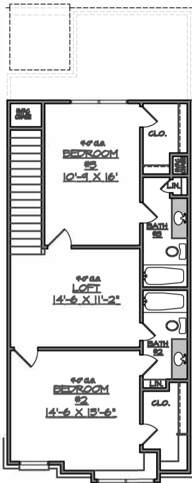
SECOND LEVEL FLOORPLAN END UNIT
